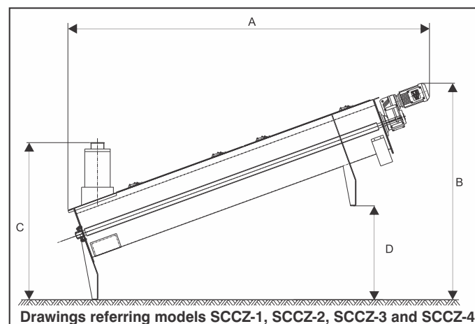
Drawings referring models SCCZ-1, SCCZ-2, SCCZ-3 and SCCZ-4
